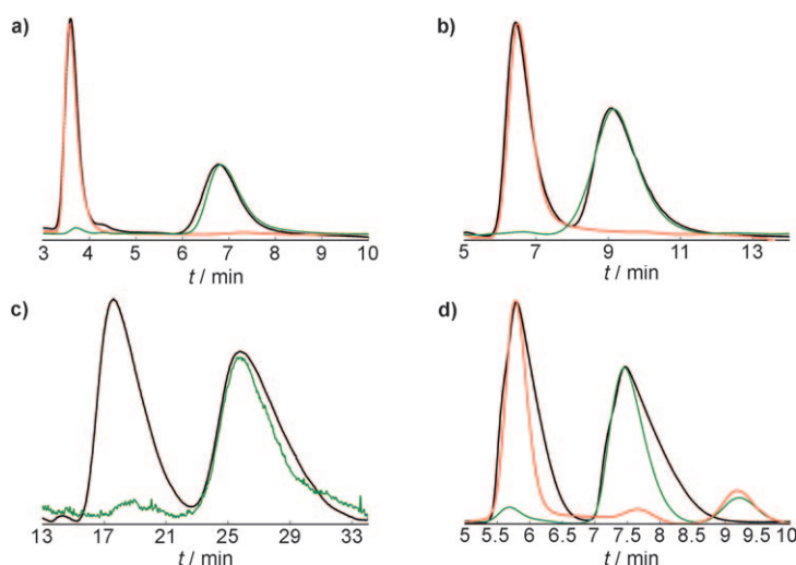
Figure 3. CSP HPLC chromatograms and enantiomeric purity control of the residual enantiomers obtained from semipreparative HPLC resolution on chiral stationary phase: black line: residual racemate, red line: first eluted residual enantiomer; green line: second eluted residual enantiomer. a) 4e , b) 4f , c) 5 , d) 2 . An achiral impurity, formed during the chromatographic resolution process together with 2-methylbenzimidazole, is visible at about 9 min. elution time.
