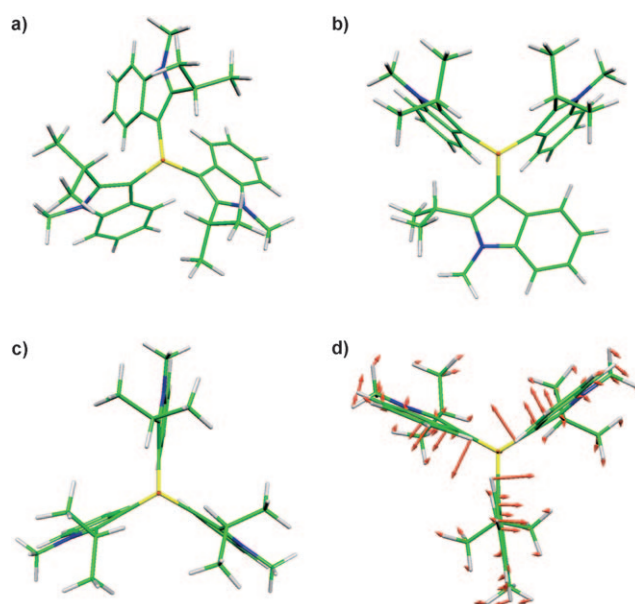
Figure 1. Selected B3LYP/cc-pVDZ optimised structures of tris[3-(1-methyl-2-isopropyl)indolyl]phosphane oxide ( 4f ). a) M_{sss} isomer; b) transition state of the M_1 isomerization from M_{sss} to P_{ssa} ; c, d) transition state of the M_0 isomerization from M_{sss} to P_{sss} : c) view from above the oxygen atom, d) view from below the phosphorus atom with arrows representing the eigenvector related to the stereomerization mode.
