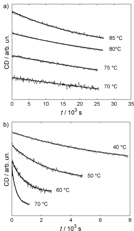
Figure 4. Variable-temperature CD decays; thin solid line: experimental; thick dashed line: best-fit. Top: 2 (solvent MeCN:water/15:85). Bottom: 4e (solvent MeCN:water/28:72). The CD curves have been vertically shifted for the sake of clarity. Note the different timescale in the two panels.
