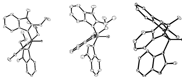
Figure 2. ORTEP presentations of a single enantiomer of: 4c (left), 4h (middle), and 5 (right).
