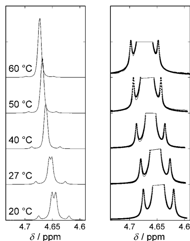
Figure 6. ^1\text{H} -DNMR experiments on 4c ( [\text{D}_6]\text{DMSO} ). Left panel: experimental spectra of the methylene protons of the methoxymethylene groups. Right panel: enlarged view of the external minor peaks; line: experimental spectra, dots: constrained best-fit spectra.
