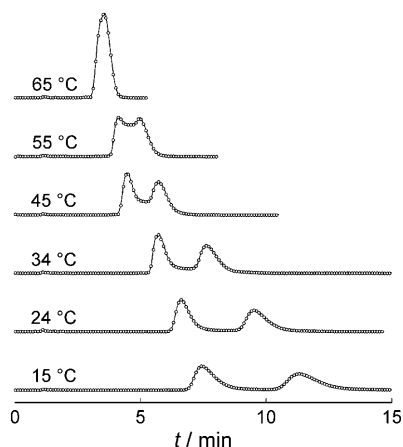
Figure 5. Variable-temperature dynamic CSP HPLC of 4c (eluant MeCN/water 2:8, flow 0.7 ccmin -1 ); open circles: experimental; solid line: best-fit.
